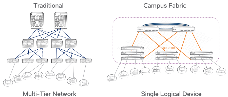
Figure 1. Ruckus Campus Fabric architecture versus a traditional multi-tier campus network.
