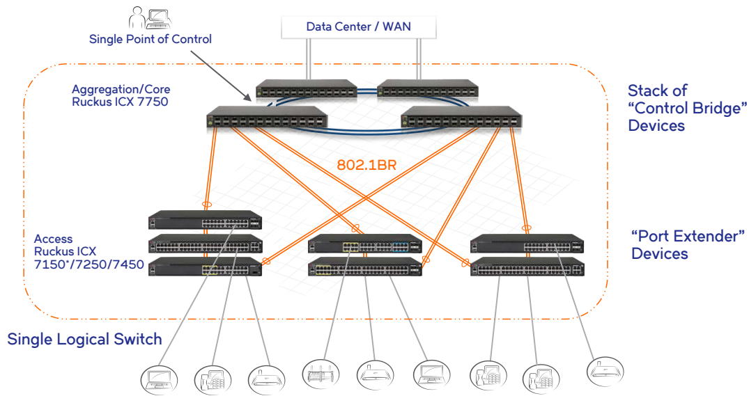
Figure 2. Ruckus Campus Fabric combines multiple network layers into a single logical device.
